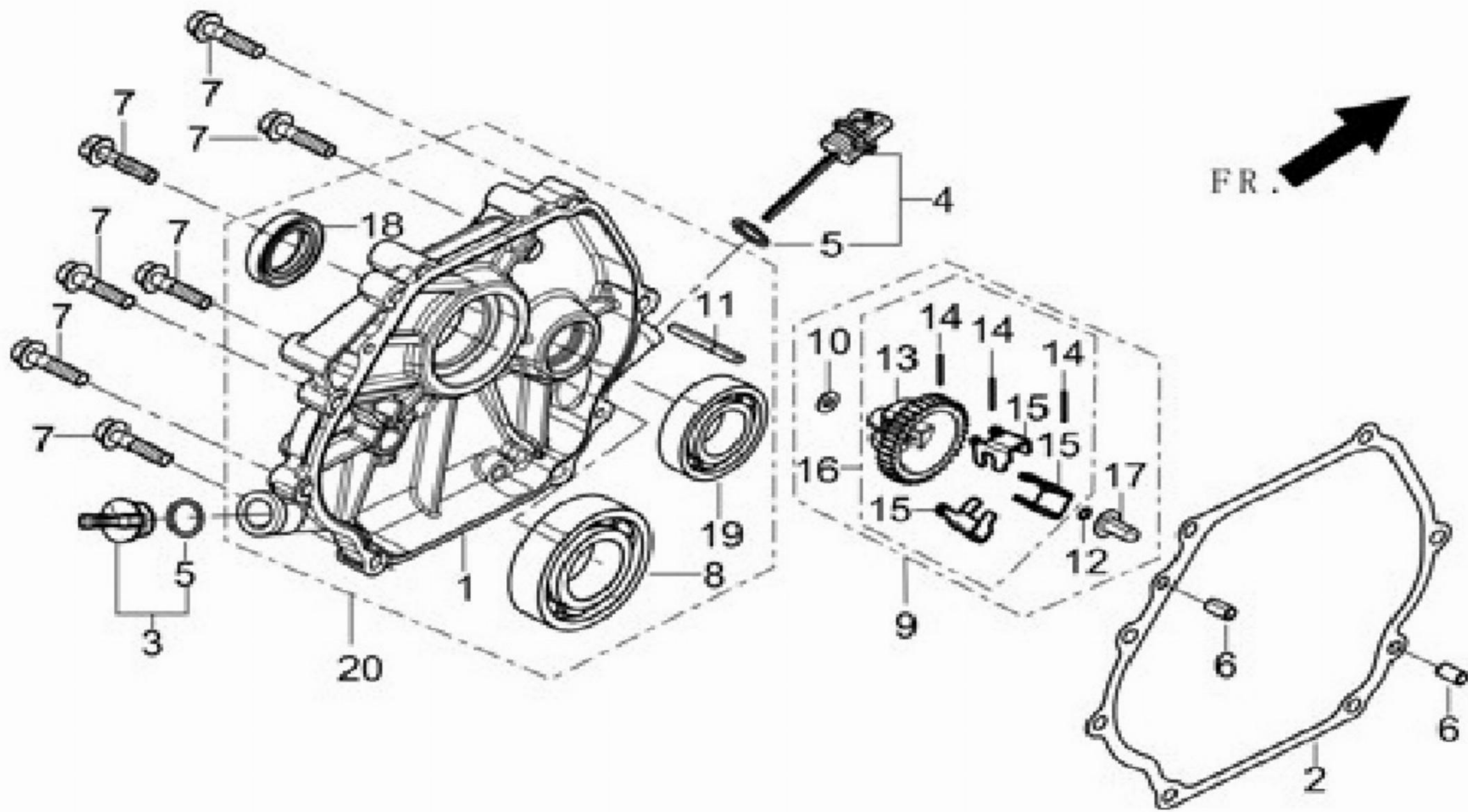
FIG.2 COVER SUBASSEMBLY, CRANKCASE / GEAR ASSY, GOVERNOR (E02)
