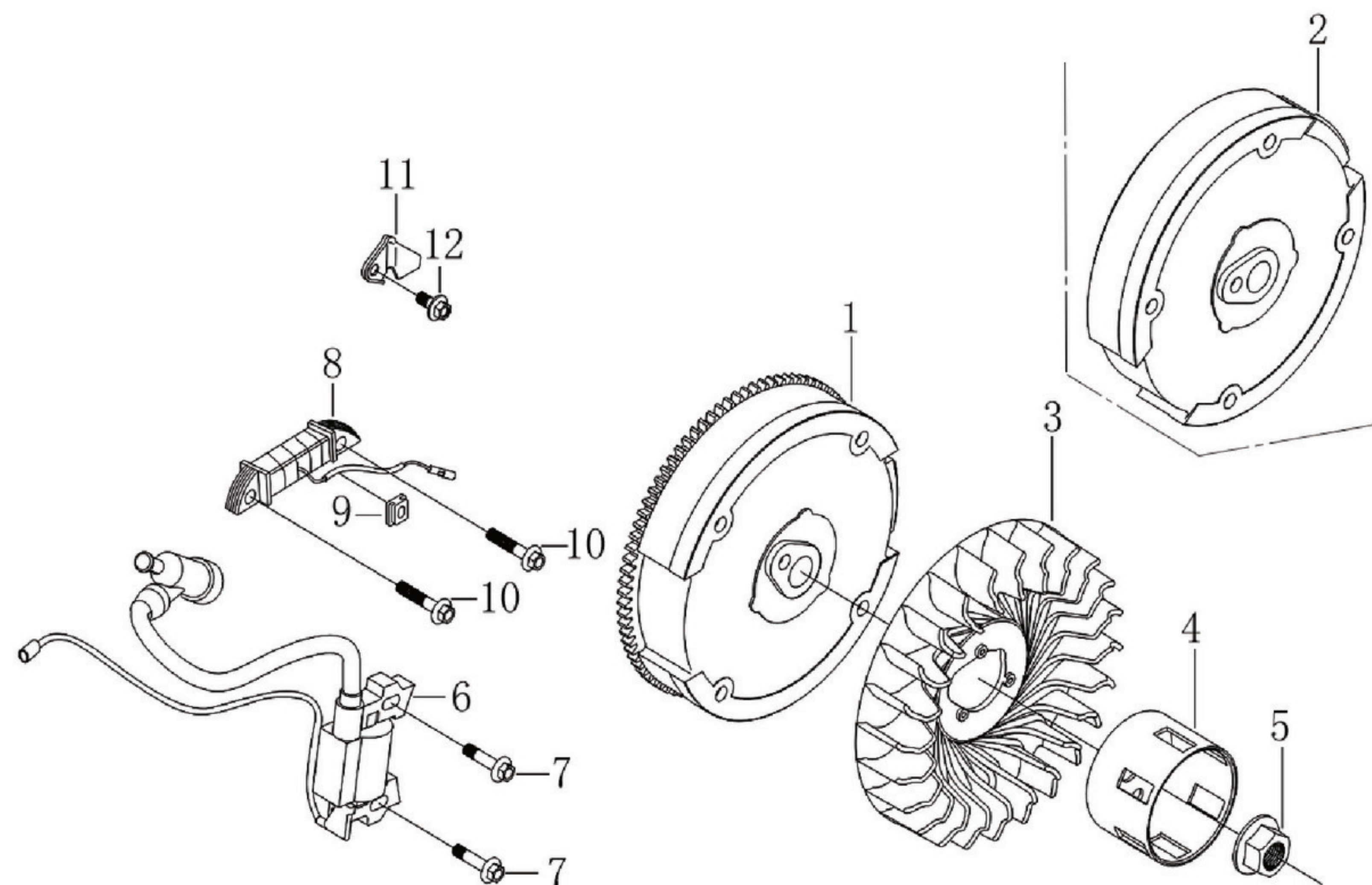
(FLYWHEEL/COIL ASSY.)
